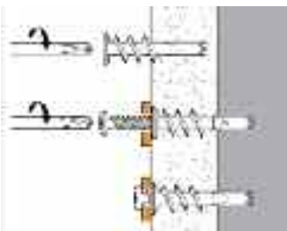
Plasterboard Anchor / Driva
