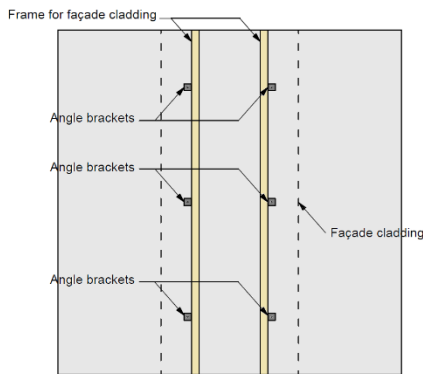
Figure 1.2 - Example of statically indeterminate fixing for the anchorage
